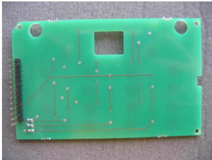
Photograph No.21 Display PCB second sideview
