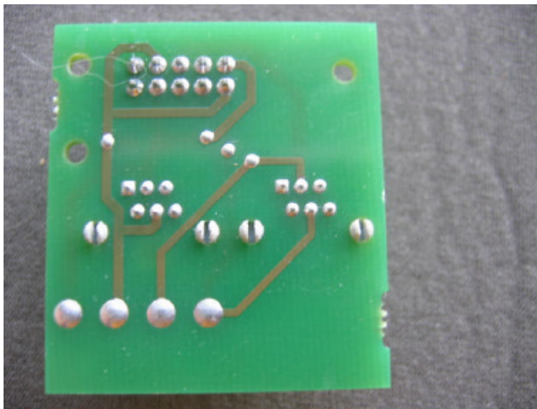
Photograph No.25 Phone line PCB second side view
